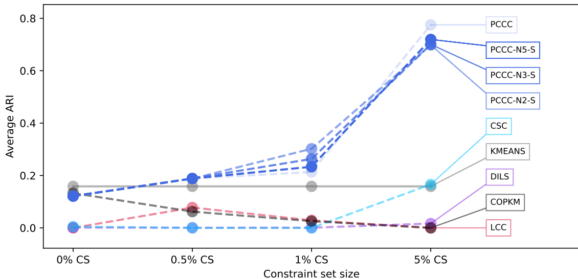
Figure 11: Adjusted Rand Index for different constraint set sizes, averaged across data sets (from collection COL3) and repetitions. Higher values indicate more overlap with the ground truth assignment. All versions of the PCCC algorithm consistently outperform the state-of-the-art algorithms. Note that we replaced nan values with an ARI value of 0 before computing the averages.
