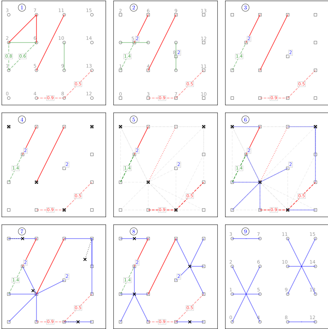
Figure 3: Illustrations for flowchart based on the illustrative example. The input consists of n = 16 objects that are described by 2 features. The goal is to partition this data set into k = 4 clusters. The additional information consists of three hard cannot-link constraints, two hard must-link constraints, two soft cannot-link constraints, and two soft must-link constraints. The algorithm is applied with parameter q = 2 , which explains why the hard cannot-link constraint between the contracted nodes 4 and 9 can be omitted in the assignment step (see illustrations 5 and 6).
