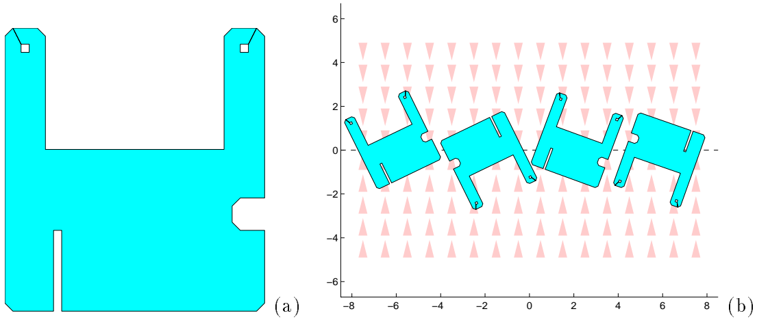
Figure 21: Sample part: (a) nonconvex shape with holes; (b) its four stable equilibria in a unit squeeze field.
