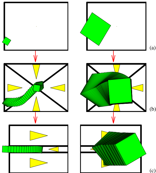
Figure 1: Sensorless sorting using programmable force vector fields: parts of different sizes are first centered and subsequently separated depending on their size.
