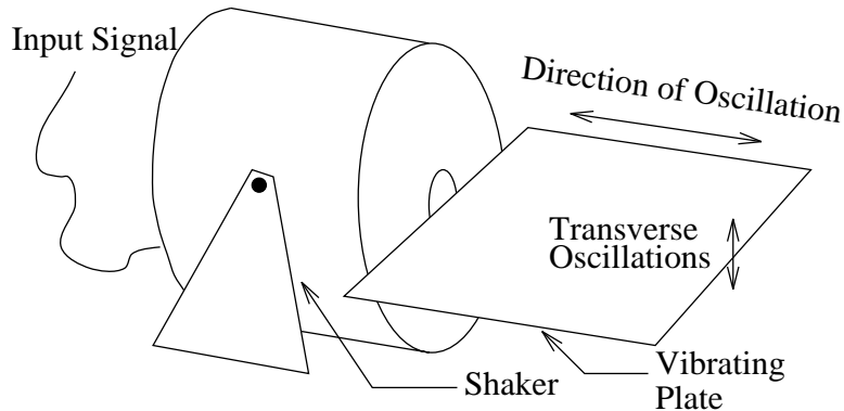
Figure 2: Schematic of experimental setup 1: A 50\text{ cm} \times 40\text{ cm} aluminum plate is forced to oscillate horizontally by the shaker armature. The forced oscillation causes a transverse vibration of the plate.
