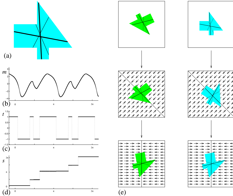
Figure 10: (a) Polygonal part. Stable (thick line) and unstable (thin line) bisectors are also shown. (b) Moment function. (c) Turn function, which predicts the orientations of the stable and unstable bisectors. (d) Squeeze function, constructed from the turn function. (e) Alignment strategy for two arbitrary initial configurations. See URL http://www.cs.cornell.edu/home/karl/Cinema for an animated simulation.
