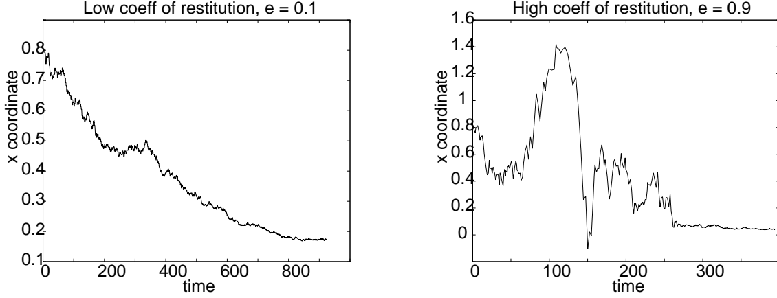
Figure 26: Simulation results showing the position of a particle moving on a vibrating string.
