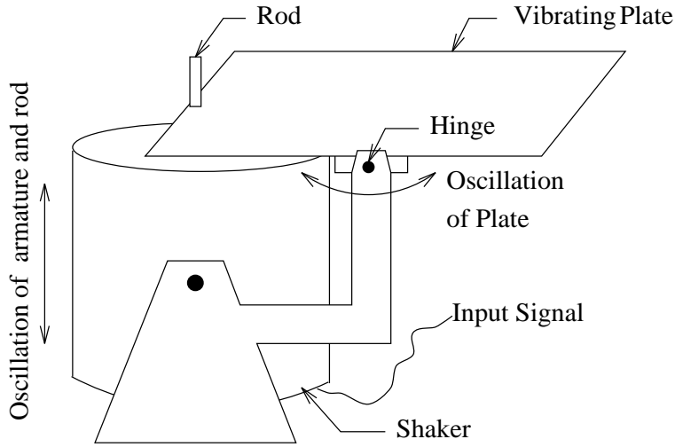
Figure 3: Schematic of experimental setup 2: The aluminum plate is hinged and can oscillate about an axis in its middle.
