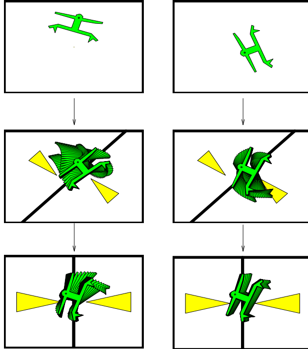
Figure 8: Sensorless parts orienting using force vector fields: The part reaches unique orientation after two subsequent squeezes. There exist such orientating strategies for all polygonal parts. See URL http://www.cs.cornell.edu/home/karl/MicroManipulation for an animated simulation.
