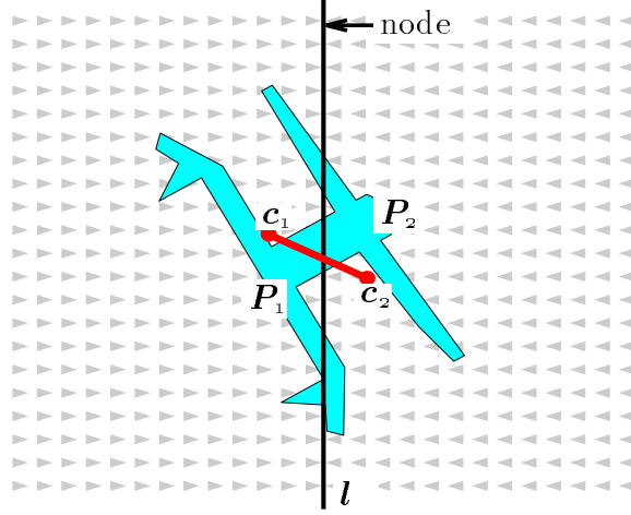
Figure 9: Equilibrium condition: To balance force and moment acting on P in a unit squeeze field, the two areas P_1 and P_2 must be equal (i.e., l must be a bisector), and the line connecting the centers of area c_1 and c_2 must be perpendicular to the node line.
