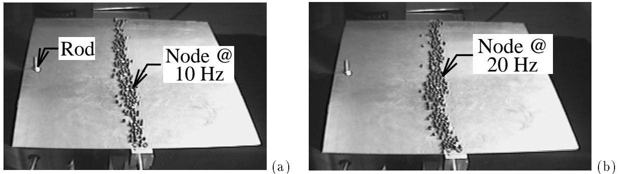
Figure 5: Experimentally determined vibrational nodes at (a) 10 Hz and (b) 20 Hz , for experimental setup 2 (see Figure 3).
