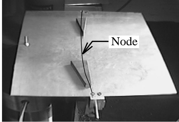
Figure 7: Stable position of planar parts in experimental setup 2, at a frequency of 20 Hz. The node is marked according to Figure 5.
