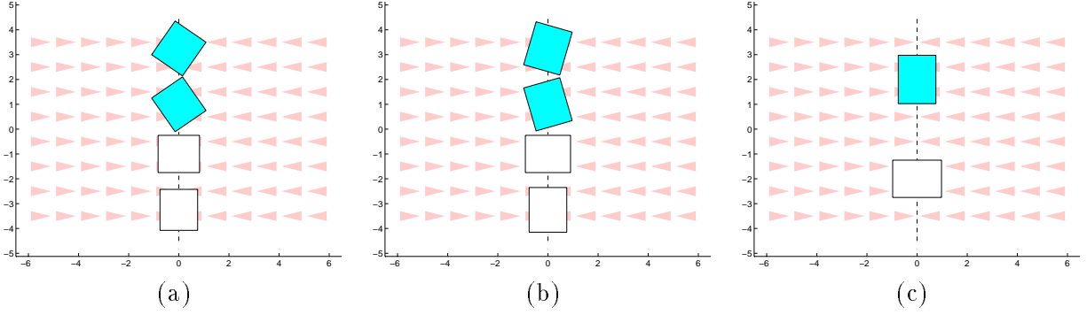
Figure 14: Stable (dark) and unstable (white) equilibria of three rectangular parts in a unit squeeze field with vertical squeeze line: (a) R_{10} , edge ratio 1.1; (b) R_{20} , edge ratio 1.2; (c) R_{30} , edge ratio 1.3. R_{10} and R_{20} exhibit two stable equilibria, R_{30} exhibits only one.
