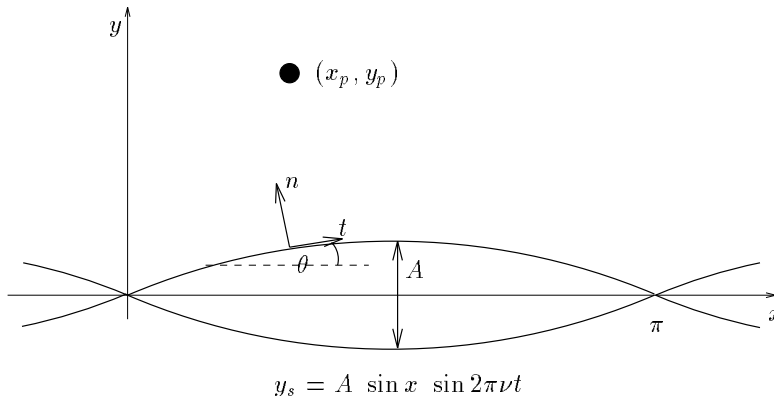
Figure 25: Particle bouncing on a vibrating string.
