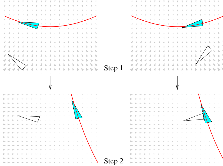
Figure 17: Manipulation vocabulary for a triangular part on a vibrating plate, consisting of two consecutive force fields with slightly curved nodal lines (attractors) which bring the part into (approximately) the same equilibria.
