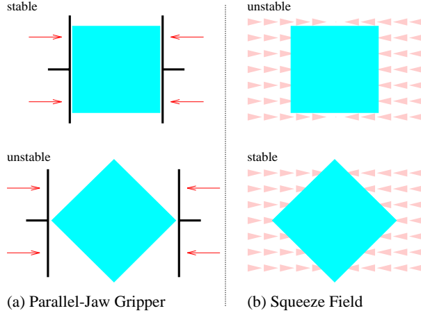
Figure 11: Equilibrium configurations for a square-shaped part using (a) a frictionless parallel-jaw gripper and (b) a MEMS squeeze field. In this example, stable and unstable equilibria are reversed.
