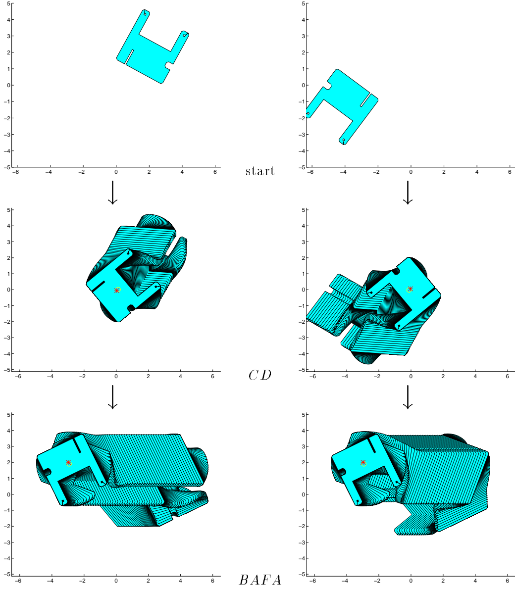
Figure 23: Two sample executions of the manipulation grammar strategy CD BA AF FA . For clarity, the simulation trace has been broken up into parts: initial pose (top), motion under CD (middle), and motion under BA AF FA (bottom). Initial poses: (a) \mathbf{z}_0 = (2, 2, -0.5) , (b) \mathbf{z}_0 = (-4, -1, 2.5) . Final pose \mathbf{e}_* \approx (-2.9, 1.9, 3.6) .
