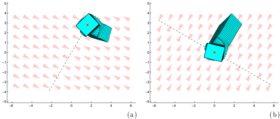
Figure 19: Simulation of part R_{20} from equilibrium 3 by using finite field operator CD , reaching equilibrium 6: (a) applying field C ; (b) applying field D .
