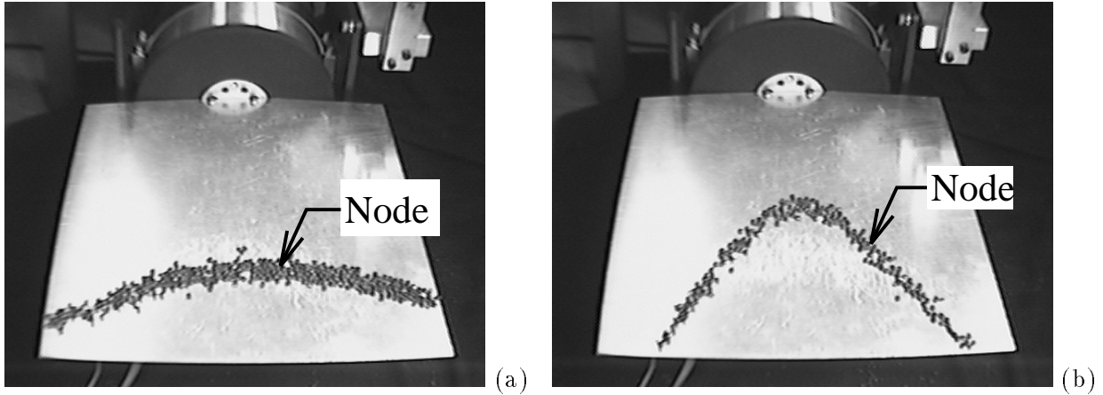
Figure 4: Experimentally determined nodes at (a) 60 Hz and (b) 100 Hz , for experimental setup 1 (see Figure 2). After vibrating the plate for a short time, the particles form Chladni figures, which indicate the location of the vibrational nodes.
