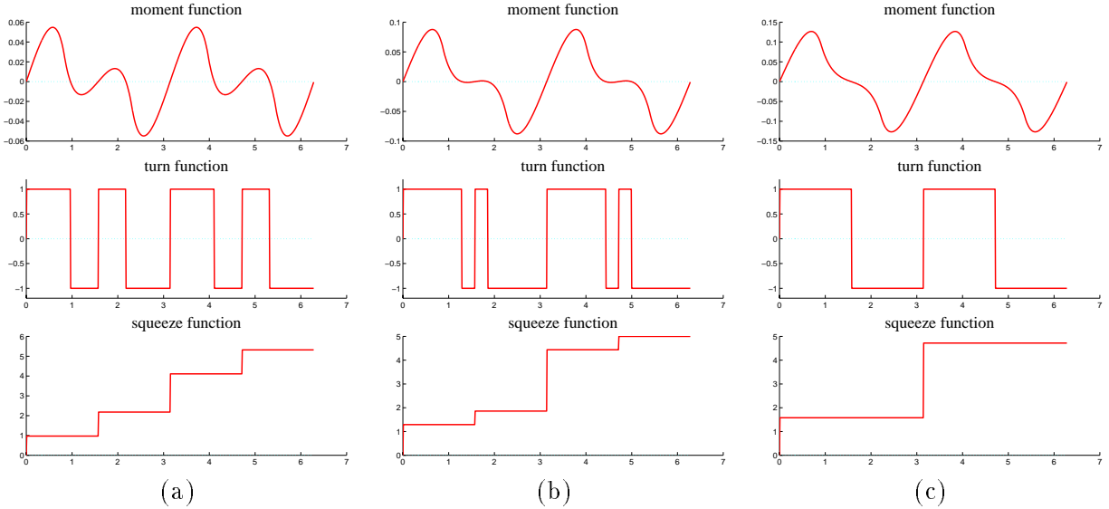
Figure 15: Moment function, turn function, and squeeze function for three rectangular parts: (a) R_{10} , edge ratio 1.1; (b) R_{20} , edge ratio 1.2; (c) R_{30} , edge ratio 1.3. R_{10} and R_{20} exhibit two stable equilibria for \theta in the range [0 \dots \pi] , R_{30} exhibits only one.
