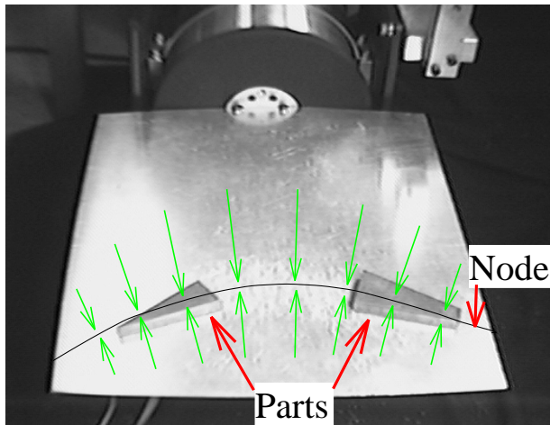
Figure 6: Stable position of planar parts in experimental setup 1, at a frequency of 60 Hz. The node is marked according to Figure 4.
