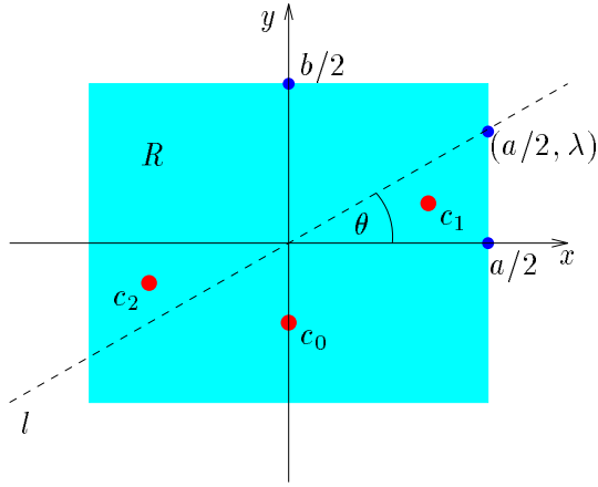
Figure 13: Analytically determining the moment function for a rectangular part R with sides of length a and b . c_0 is the center of mass of the segment below the x -axis. c_1 and c_2 are the centers of the triangular segments between x -axis and line l .
