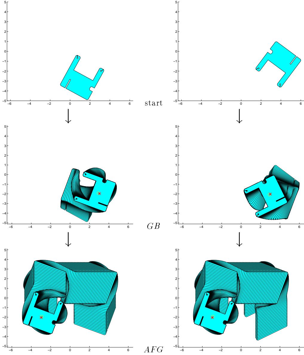
Figure 24: Two sample executions of strategy GB\ BA\ AF\ FG = GBAFG . For clarity, the simulation trace has been broken up into parts: initial pose (top), motion under GB (middle), and motion under AFG (bottom). Initial poses: (a) \mathbf{z}_0 = (1, -3, -0.5) , (b) \mathbf{z}_0 = (4, -1, 2.5) . Final pose \mathbf{e}_* \approx (-2.9, -1.9, 5.9) .
